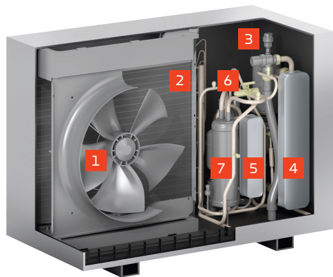
Outdoor unit 2.1 to 8.0 kW (A7/W35)
